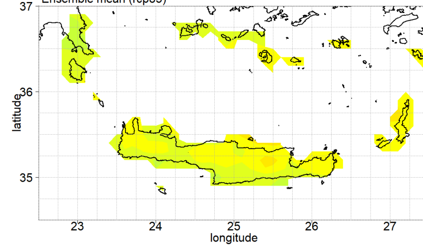
Number of Days with FWI>30 (Days/year) Change Between 2021-2040 and 1981-2000 Ensemble mean (rcp85)
