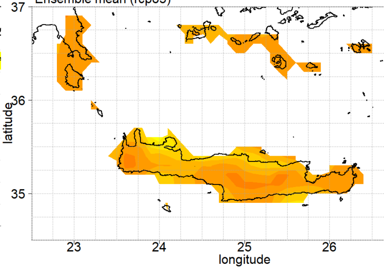
Number of Days with FWI>30 (Days/year) Change Between 2041-2060 and 1981-2000 Ensemble mean (rcp85)
