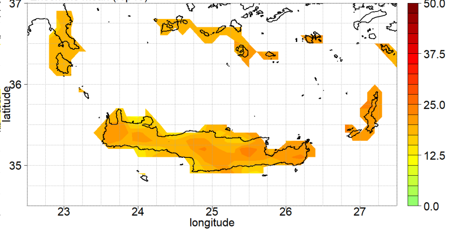
Number of Days with FWI>30 (Days/year) Change Between 2081-2100 and 1981-2000 Ensemble mean (rcp45)
